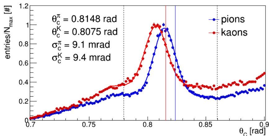
LUT Version 12 photons generated over the full end of the bar surface
