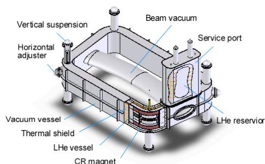
Figure 3: Cryostat structure of a CR dipole
