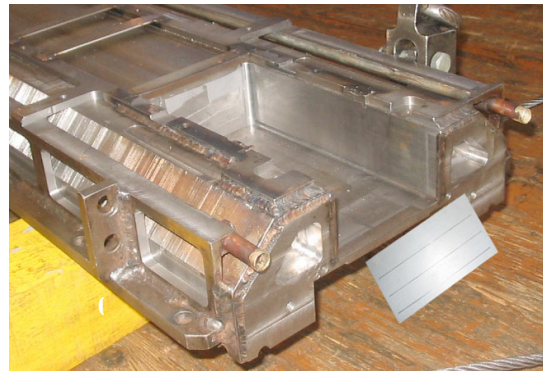
Figure 2: Preparation of the SIS100 test model PDP2 with improved yoke ends (laser-cut slits, reduced stainless steel end plate and minimized brackets).
