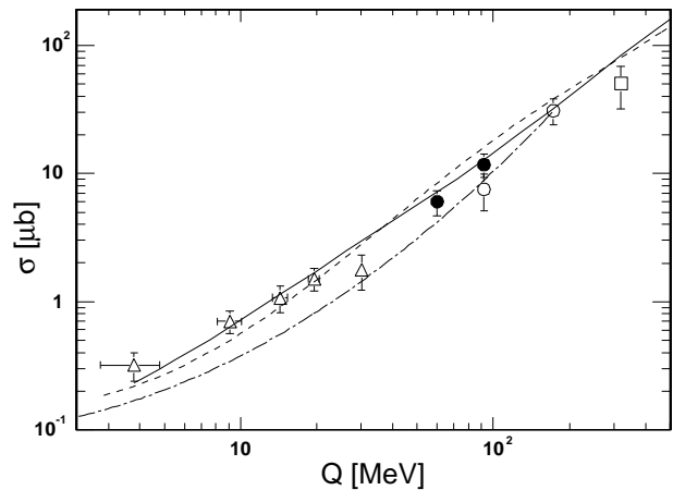
Fig. 9. Experimental data on the pp \rightarrow pp\omega total cross section shown in Fig. 8 compared with the predictions from microscopic theoretical models shown by the chain ([3]), solid ([4]), and dashed ([5]) curves.
