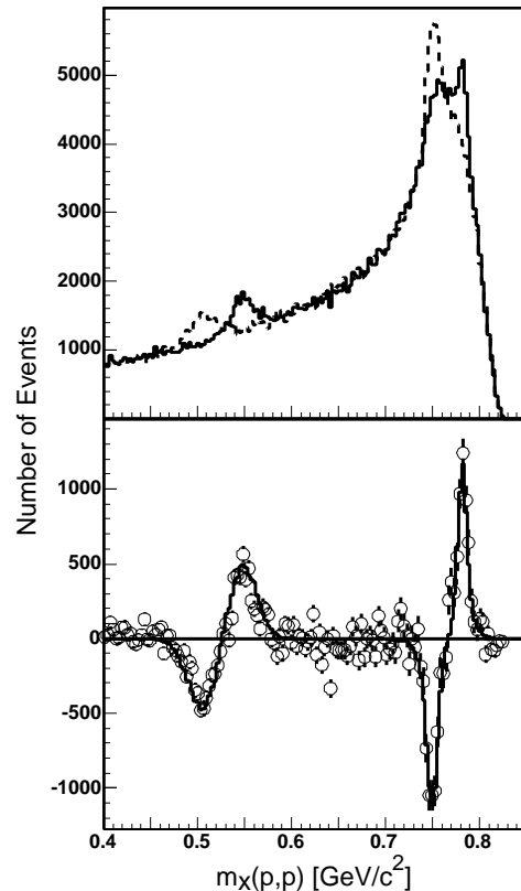
Fig. 4. Upper frame: The missing-mass distribution of the pp \rightarrow ppX reaction in bins of 3 \text{ MeV}/c^2 measured at 2.85 \text{ GeV}/c (solid line, Fig. 3a) is shown together with the analogous distribution obtained at 2.95 \text{ GeV}/c (Fig. 3b) and kinematically transformed to the 2.85 \text{ GeV}/c (dashed line), as described in the text. Lower frame: The bin-by-bin difference of these two distributions is represented by points. The solid lines show simulations of the pp \rightarrow pp\eta and pp \rightarrow pp\omega reactions convoluted with acceptance. The widths of the peaks, which are strongly influenced by effects of momentum reconstruction, are very well reproduced.
