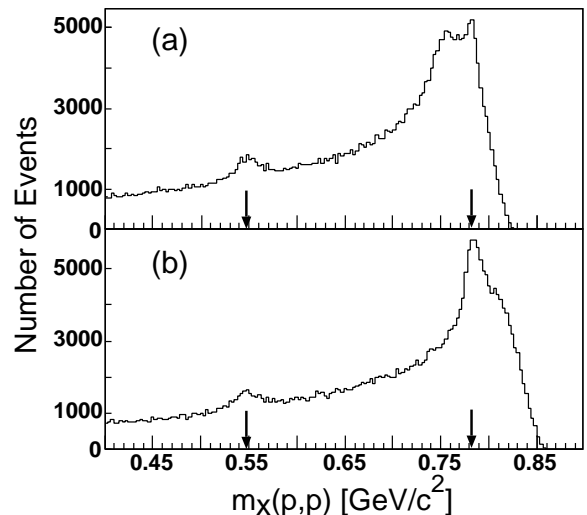
Fig. 3. The missing-mass distributions of the pp \rightarrow ppX reaction in bins of 3 MeV/c 2 measured (a) at 2.85 GeV/c and (b) at 2.95 GeV/c. There is clear evidence for peaks corresponding to the production of both the \eta and \omega (indicated by arrows) but sitting on a large background.
