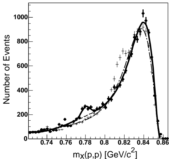
Fig. 7. Missing-mass distribution of the pp \rightarrow ppX reactions in bins of 4 \text{ MeV}/c^2 obtained at Q = 92 \text{ MeV} in the 10 < \varepsilon_{pp} < 30 \text{ MeV} range (closed circles) is shown together with the corresponding transformed distribution (crosses). The thick solid line represents the fit result for the measured spectrum. The dashed and dashed-dotted lines show two extreme cases of the background behaviour. The maximum systematic error was established to be 25%.
