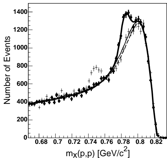
Fig. 5. The missing-mass distribution of the pp \rightarrow ppX reaction in bins of 3 MeV/c 2 obtained at 2.85 GeV/c within a restricted part of the total acceptance (closed circles) is shown together with the corresponding distribution kinematically transformed from the 2.95 GeV/c to 2.85 GeV/c (crosses). The thick solid line represents a fit to the distribution at 2.85 GeV/c while the thin one shows the background function under the \omega peak found in this case. The same fit procedure was applied to the transformed distribution and the resulting background function shown by the dashed line.
