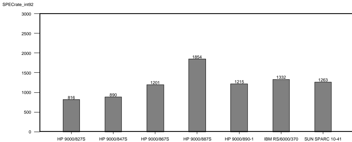
Figure 7 SPECrate_int92 Results for Competitive Systems
