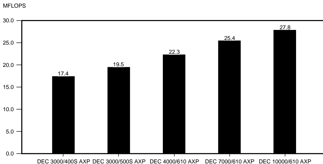
Figure 20 Livermore Loops Results for Alpha AXP Servers
