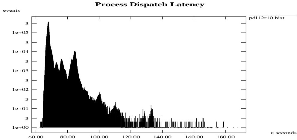
Figure 21 Basic Real-Time Primitives Process Dispatch Latency Results
