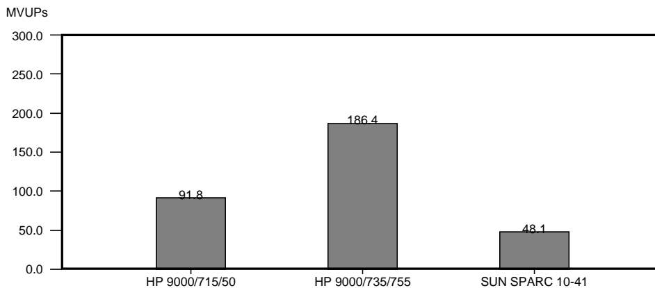
Figure 19 DN&R Labs CPU2 Results for Competitive Systems
