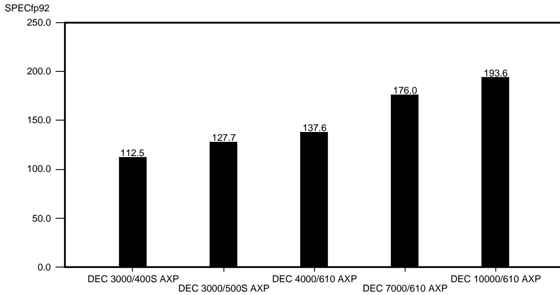
Figure 5 SPEC CFP92 Results for Competitive Systems
