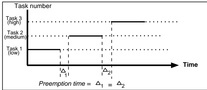
Figure 24 Rhexalstone Component-Preemption Time
