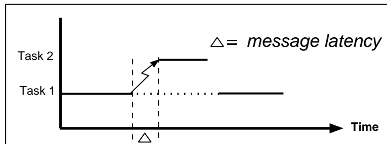
Figure 26 Rhealstone Component–Intertask Message Latency
