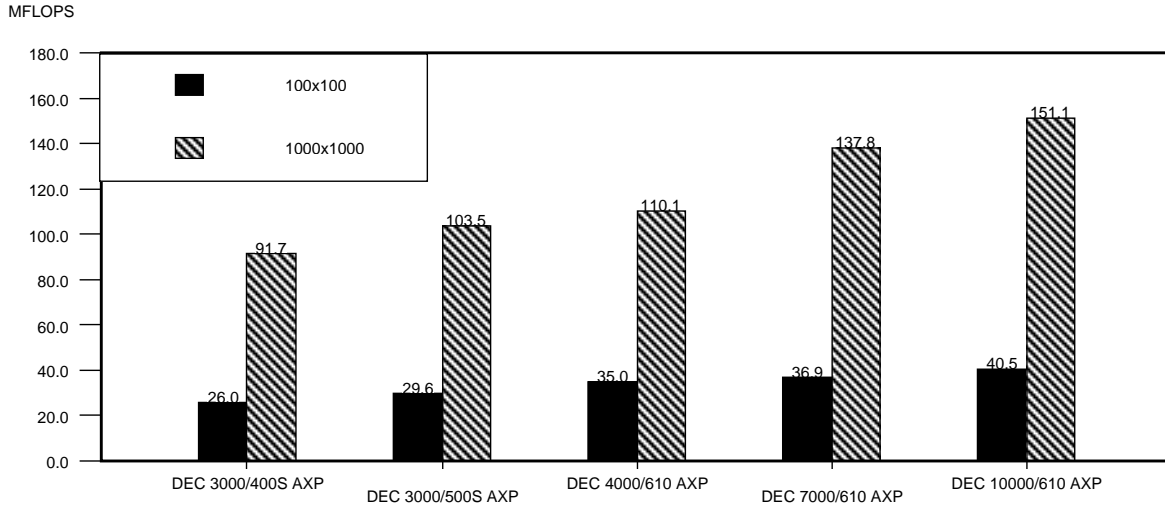
Figure 14 LINPACK Double-Precision Results for Alpha AXP Servers
