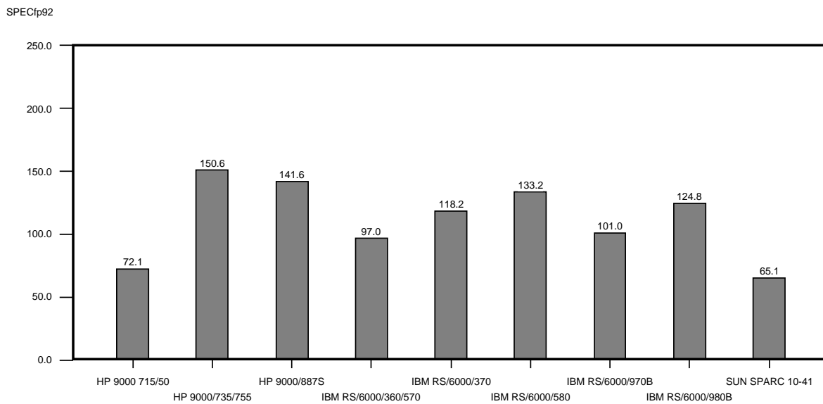
Figure 5 SPEC CFP92 Results for Competitive Systems
