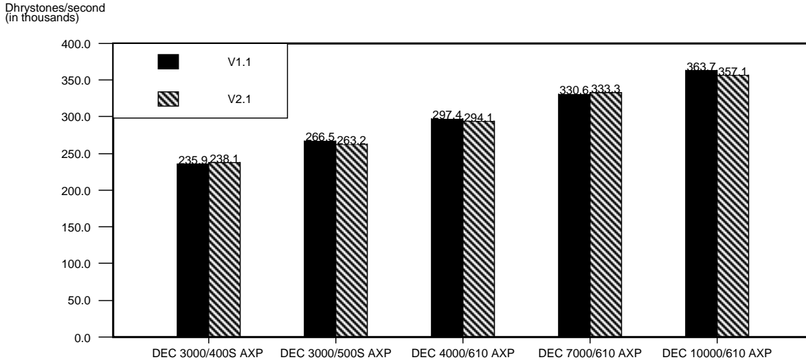
Figure 12 Dhrystone V1.1 and V2.1 Results for Alpha AXP Servers
