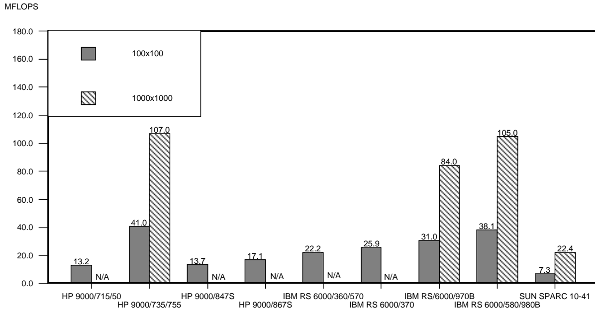
Figure 15 LINPACK Double-Precision Results for Competitive Systems
