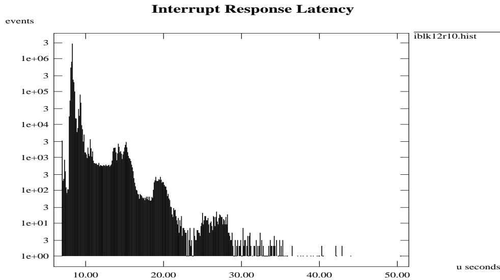
Figure 22 Basic Real-Time Primitives Interrupt Response Latency Results
