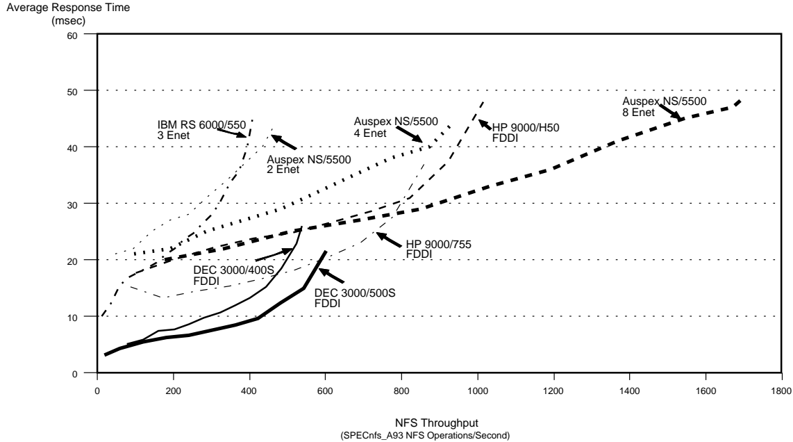
Figure 1 SPEC SFS Release 1.0 NFS Server Response Time vs. Throughput
