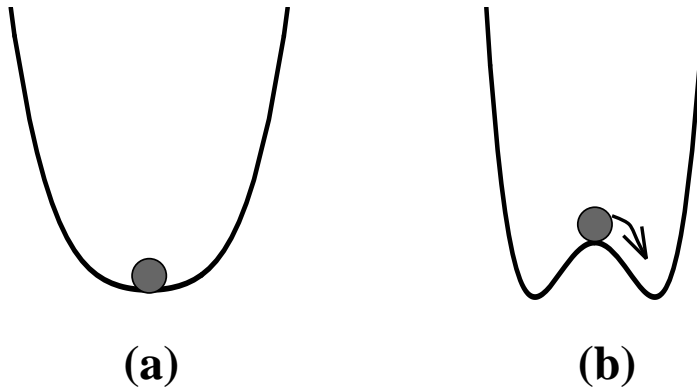
Figure 10: System in restored phase (a) and in quench scenario (b).
