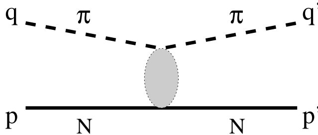
Figure 4: Pion nucleon scattering amplitude.
