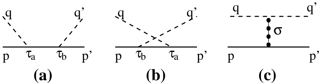
Figure 5: Diagrams contributing to the pion-nucleon scattering amplitude T_{ab} .
