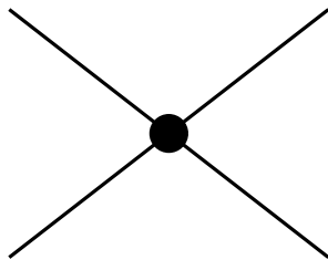
Figure 6: Leading order diagram for \pi - \pi scattering.
