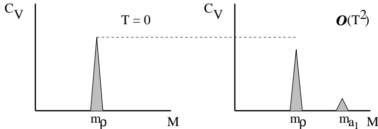
Figure 8: Vector-spectral functions at T = 0 and to leading order in temperature as given by equ. (187).
