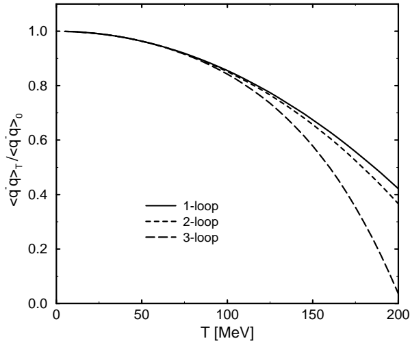
Figure 7: Temperature dependence of the quark condensate from chiral perturbation theory (chiral limit).
