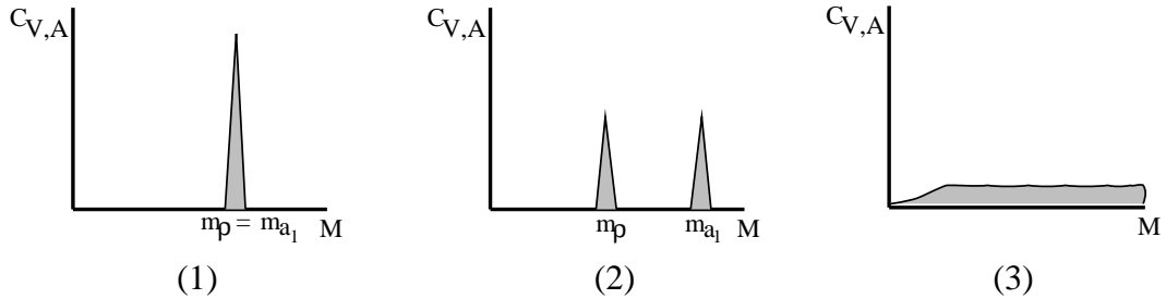
Figure 9: Several possibilities for the vector and axial-vector spectral functions in the chirally restored phase.
