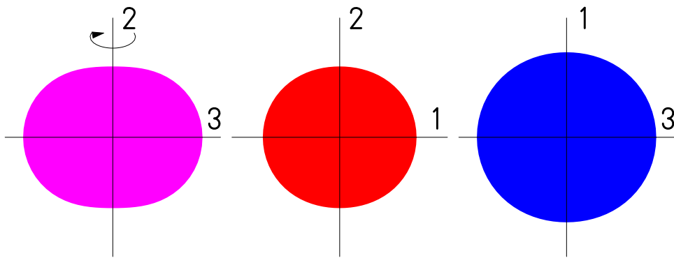
Nuclear shape with \gamma = 30^\circ and \beta = 0.3
