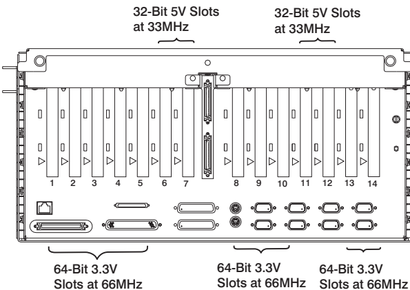
I/O Drawer Rear View with Numbered Slots
