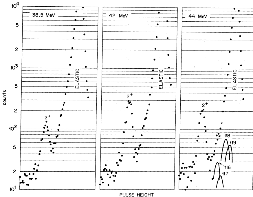
FIG. 2. Examples of ^{16}\text{O} spectra observed in an annular silicon surface-barrier detector when the beam struck a thin ^{120}\text{Sn} target.
