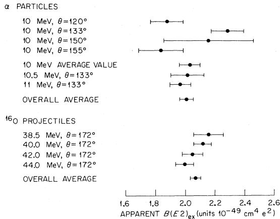
FIG. 3. Graphical summary of "apparent" B(E2) values obtained from the Coulomb excitation of the first 2+ state in ^{120}\text{Sn} . Results are shown for both \alpha particles and ^{16}\text{O} projectiles.
