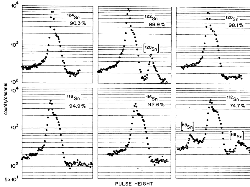
FIG. 1. Ge(Li) \gamma -ray spectra which result from the Coulomb excitation of the first 2+ state in the even tin nuclei by 45.5-MeV ^{16}\text{O} projectiles. \gamma rays were observed at an angle of 55^\circ to the beam direction. The Doppler shifts (shoulders on the high side of the peaks) are quite apparent.
