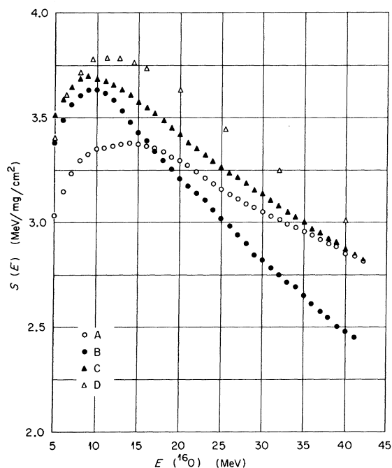
FIG. 6. Four different sets of stopping powers for ^{16}\text{O} ions in tin (see text).
