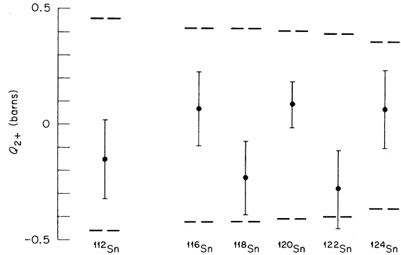
FIG. 7. The observed Q(2+) values for the different even tin nuclei. The dashed lines indicate the rotational limits (prolate and oblate). The familiar parameter \beta_2 is approximately 0.12 for the even tin nuclei.
