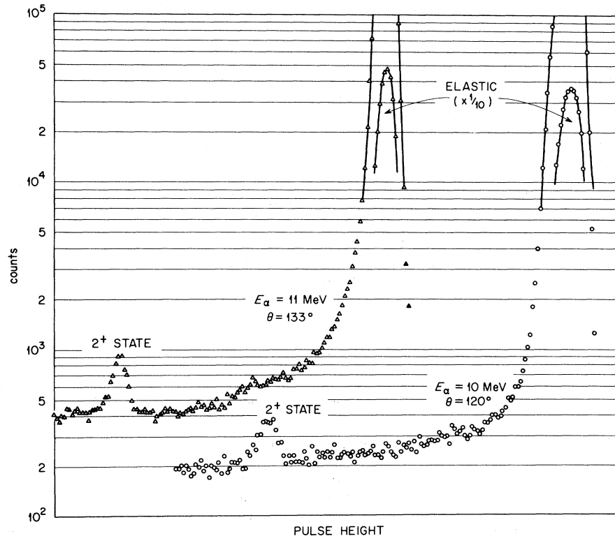
FIG. 4. Examples of \alpha -particle spectra observed in a silicon surface-barrier detector when the incident beam struck a thin ^{120}\text{Sn} target.
