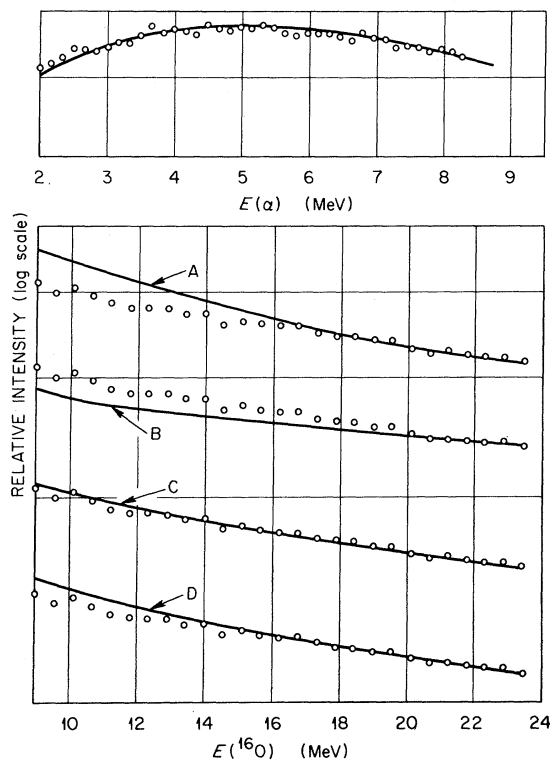
FIG. 5. Observed and calculated shapes of particle spectra backscattered from a thick ^{120}\text{Sn} target into an annular surface-barrier detector. The solid curves are calculated shapes for different shapes taken for the stopping power S(E) . The upper curve is for \alpha particles and the lower curves are for ^{16}\text{O} ions.
