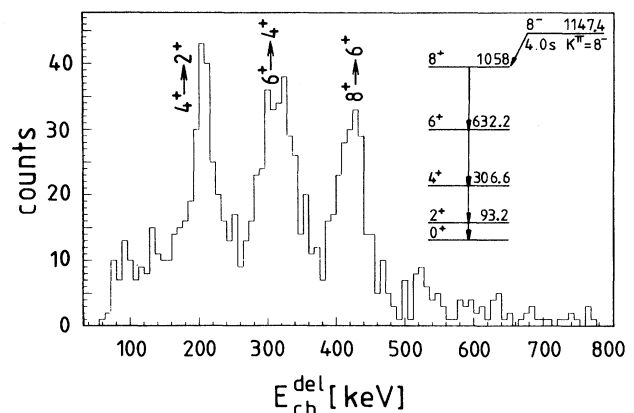
FIG. 1. Delayed \gamma ray spectrum of the Crystal Ball obtained at a bombarding energy of 590 MeV, demanding 850 \text{ keV} \leq E_{\text{sum}}^d \leq 1100 \text{ keV} and 2 \leq M_\gamma^d \leq 5 . In the right corner the partial level scheme of the \gamma ray cascade depopulating the isomer is displayed.
